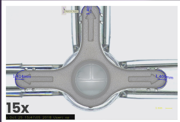
Three way IV valve mould measurement
